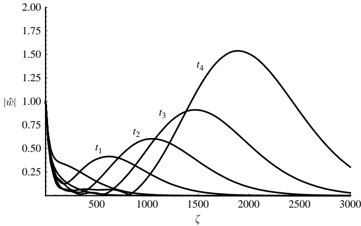
FIGURE 12. Wall-normal disturbance profiles at a succession of times at \theta = 0 , \rho = 1 and \beta/\rho = 0.007 . The latest times shown are t_1 = 2 \times 10^5 , t_2 = 3 \times 10^5 , t_3 = 4 \times 10^5 and t_4 = 5 \times 10^5 . Each profile has been normalized to unit amplitude at \zeta = 1 , so that they can be compared on the same diagram (the amplitudes increase dramatically with time due to the underlying absolute instability).
